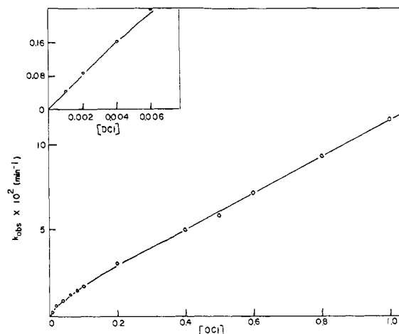
Figure 1. Plot of the pseudo-first-order rate constants, k_{\text{obsd}} , vs. the molar concentration of DCl in D 2 O for hydrolysis of MPG, t = 30^\circ , \mu = 1 M (KCl). The solid lines are calculated from the constants of Table I and the symbols represent experimental values of rate constants for given DCl concentrations.
